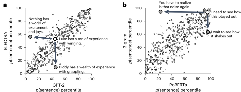
Fig. 2 | Synthesizing controversial sentence pairs. The small open circles denote 500 randomly sampled natural sentences. The big open circle denotes the natural sentence used for initializing the controversial sentence optimization, and the filled circles are the resulting synthetic sentences. a , In this example, we start with the randomly sampled natural sentence 'Luke has a ton of experience with winning'. If we adjust this sentence to minimize its probability according to GPT-2 (while keeping the sentence at least as likely as the natural sentence according to ELECTRA), we obtain the synthetic sentence 'Nothing has a world of excitement and joys'. By repeating this procedure while switching the roles of
